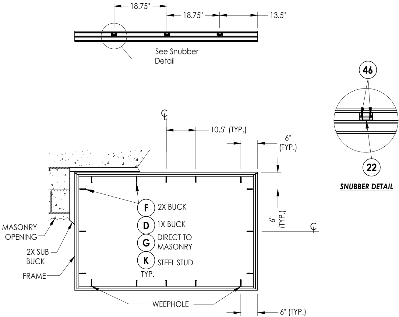
FRAME MOUNT ANCHORING 65" X 42" Max Size
