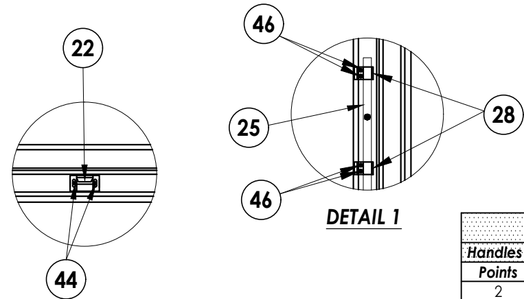
SNUBBER DETAIL
